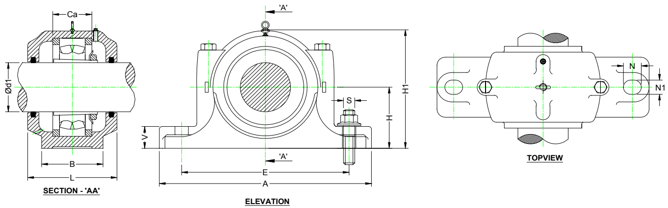
Plummer Blocks ( Bearing housings ) Series SN 500 for bearings with adapter sleeves.
